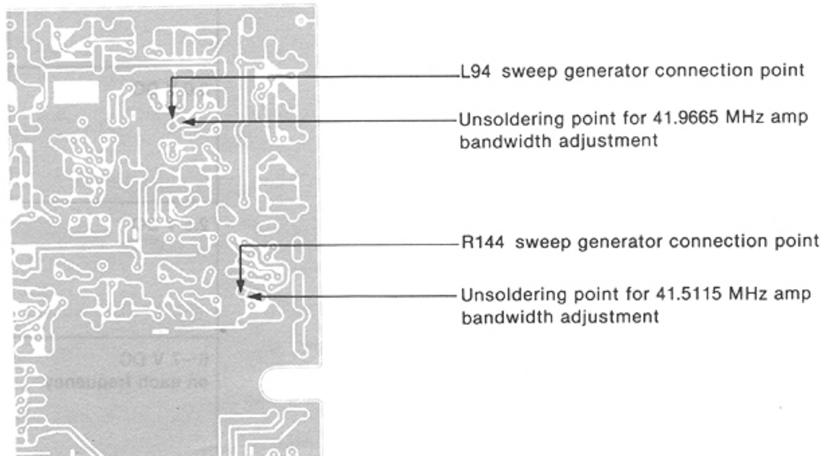
PLL-A UNIT FOIL SIDE
