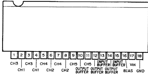
BA3812L (5-POINT GRAPHIC EQUALIZER)
