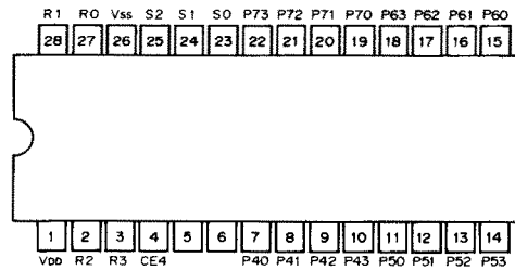
M50784SP (INPUT/OUTPUT EXPANDER)
