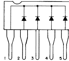
DAN401 (SWITCHING DIODE ARRAY)
